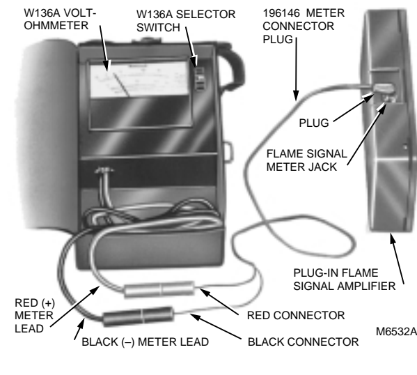
Fig. 11—Measuring microamp flame signal.
