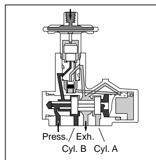
Figure 14D: Operator Pressurized
