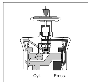
Figure 13D: Normally Open, Operator Pressurized
