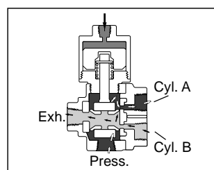
Figure 14B: Operator Pressurized
