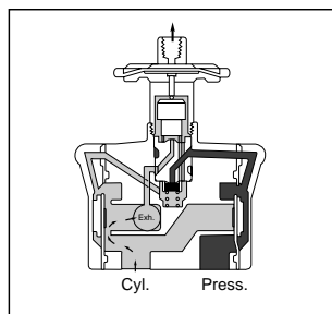
Figure 13A: Normally Closed, Operator Exhausted
