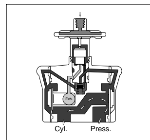
Figure 13B: Normally Closed, Operator Pressurized
