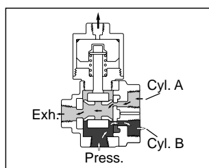
Figure 14A: Operator Exhausted
