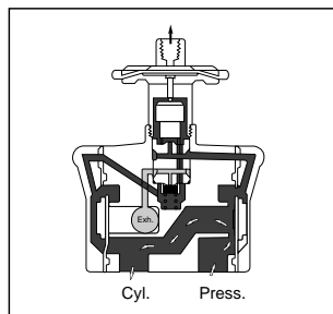
Figure 13C: Normally Open, Operator Exhausted
