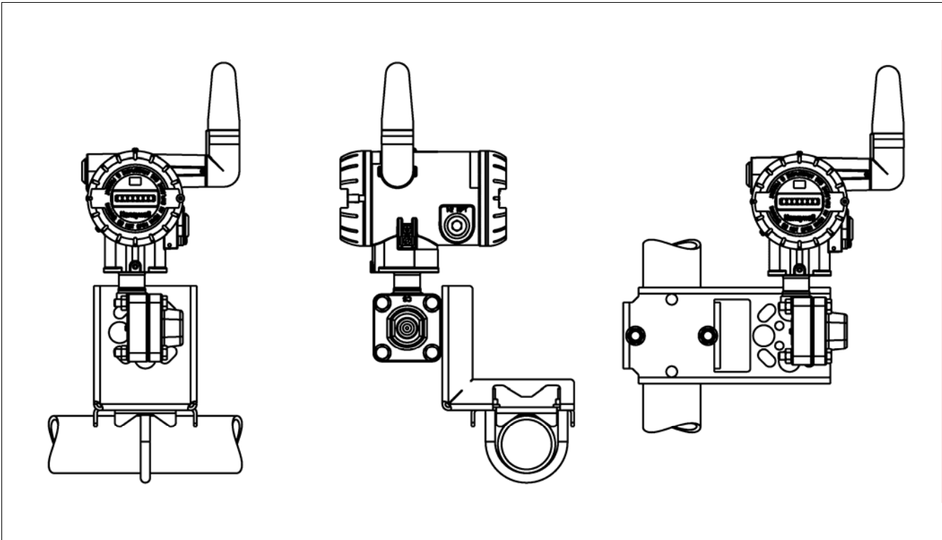
Figure 3 —Examples of typical mounting positions for dual-head models STGW944 and STGW974
